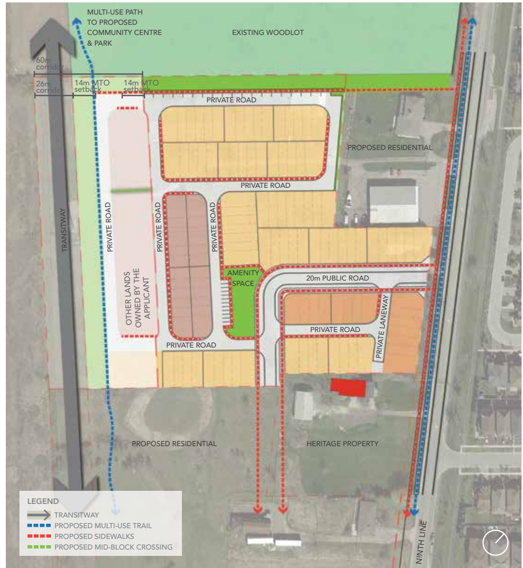
Figure 2.1e - Ninth Line South Community Pedestrian Circulation Plan
