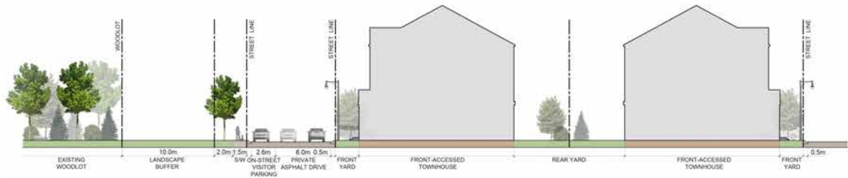
Figure 2.1n- Section E: 6m private road interface with on-street visitor parking, landscape buffer, and existing woodlot
