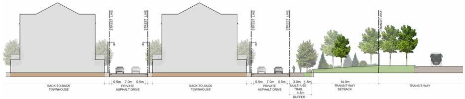
Figure 2.1m - Section D: 7m private road interface with buffer and Transitway corridor
