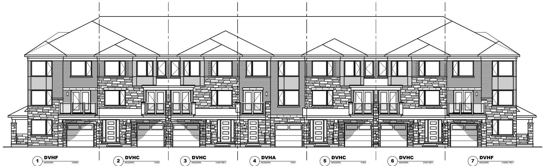
Figure 2.2b– Example of a front elevation of back-to-back townhouses.
