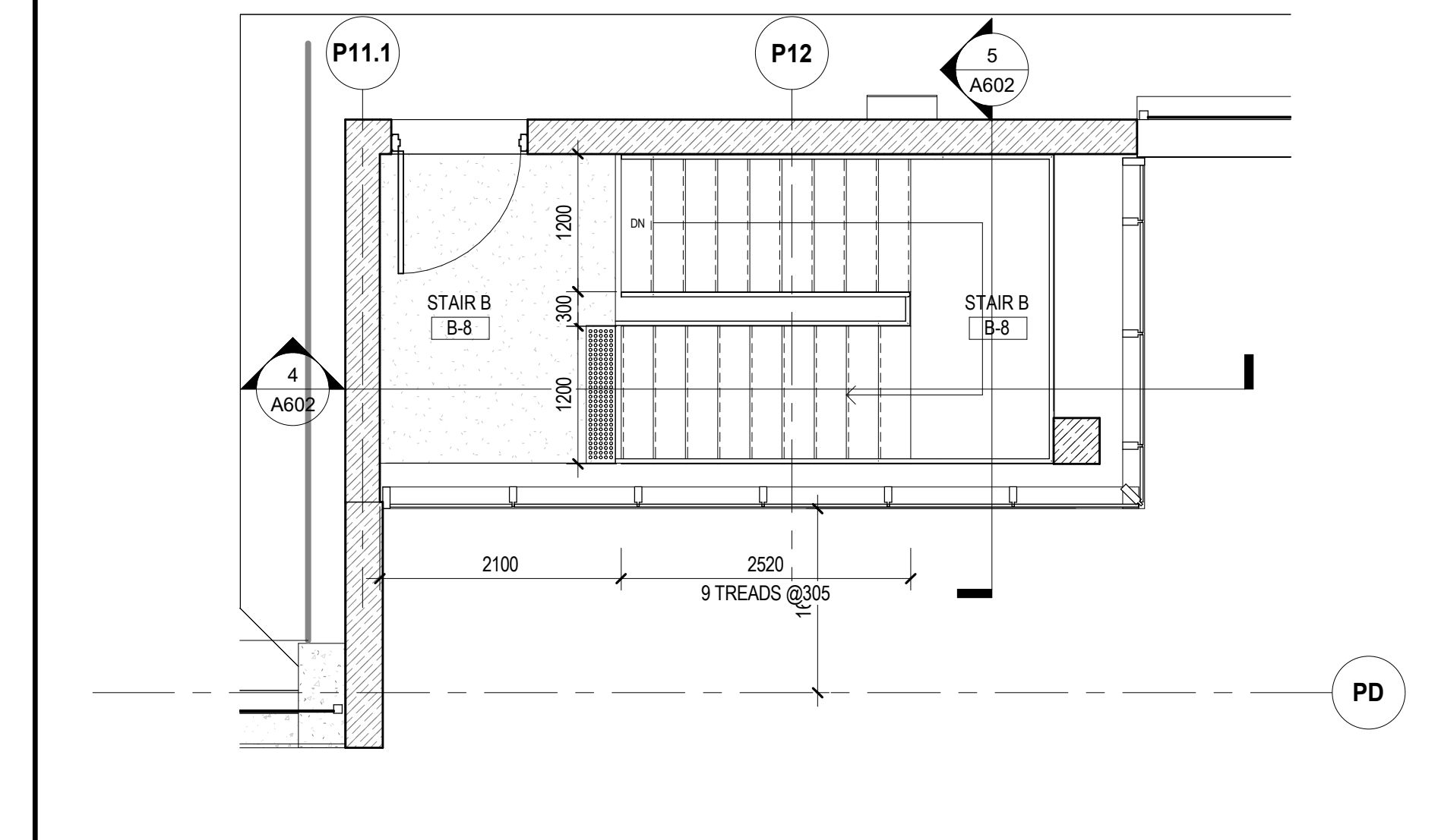
ENLARGED FLOOR PLAN - P8 - STAIR B SCALE: 1:50 A602
