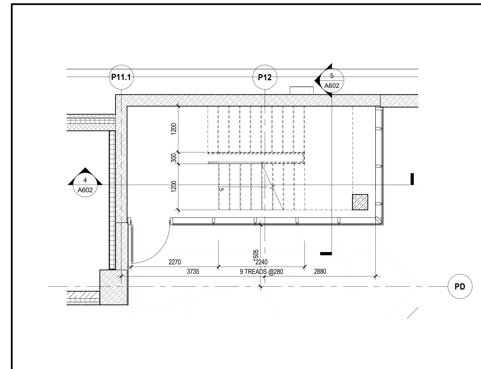
ENLARGED FLOOR PLAN - P1 - STAIR B SCALE: 1:50 A602
