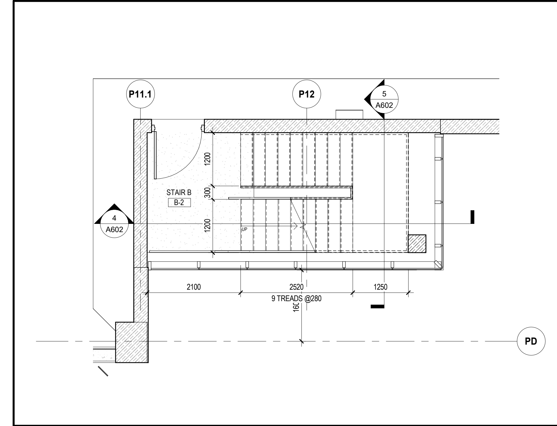
ENLARGED FLOOR PLAN - TYPICAL LEVEL - STAIR B SCALE: 1:50 A602
