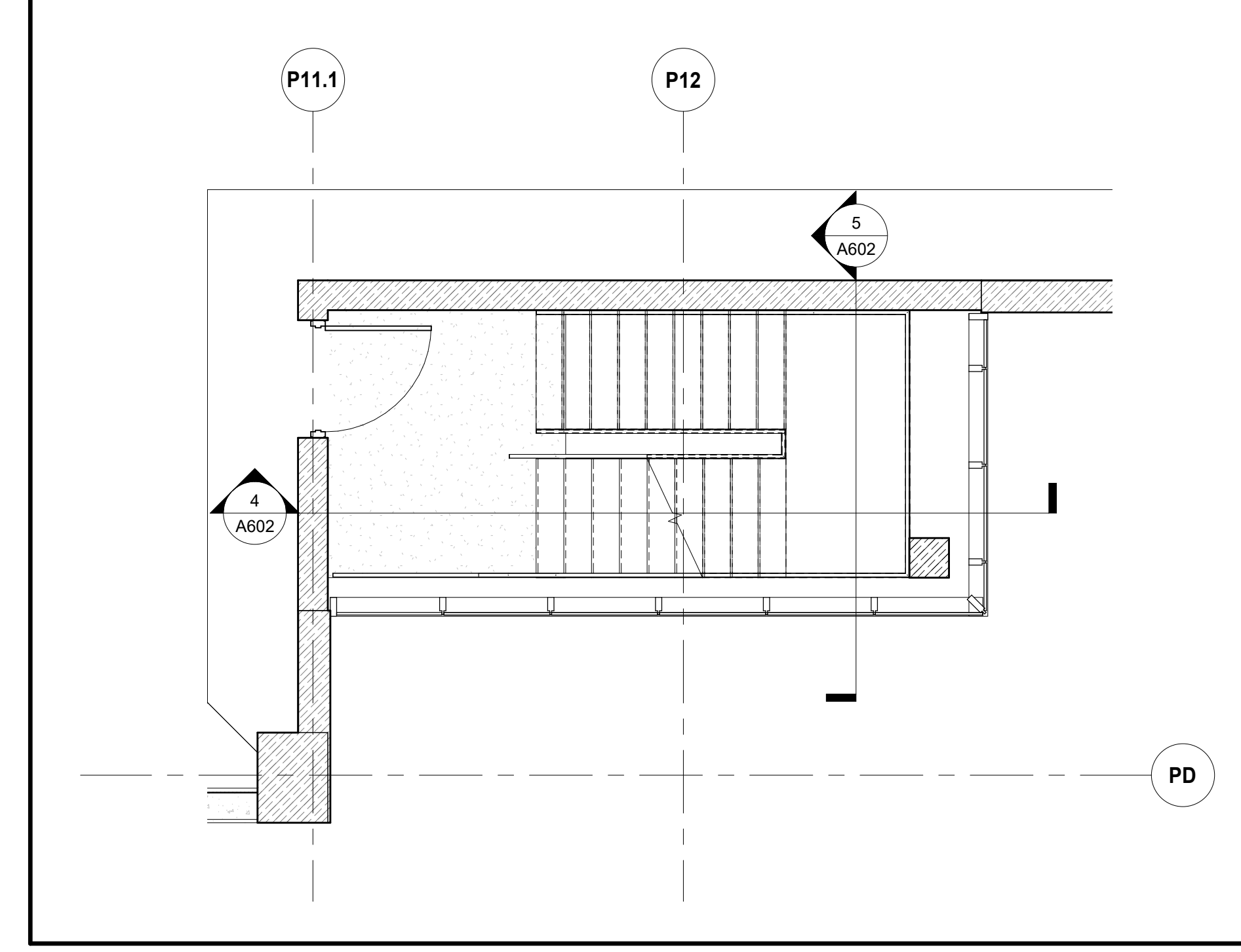
ENLARGED FLOOR PLAN - P4 & P7 - STAIR B SCALE: 1:50 A602
