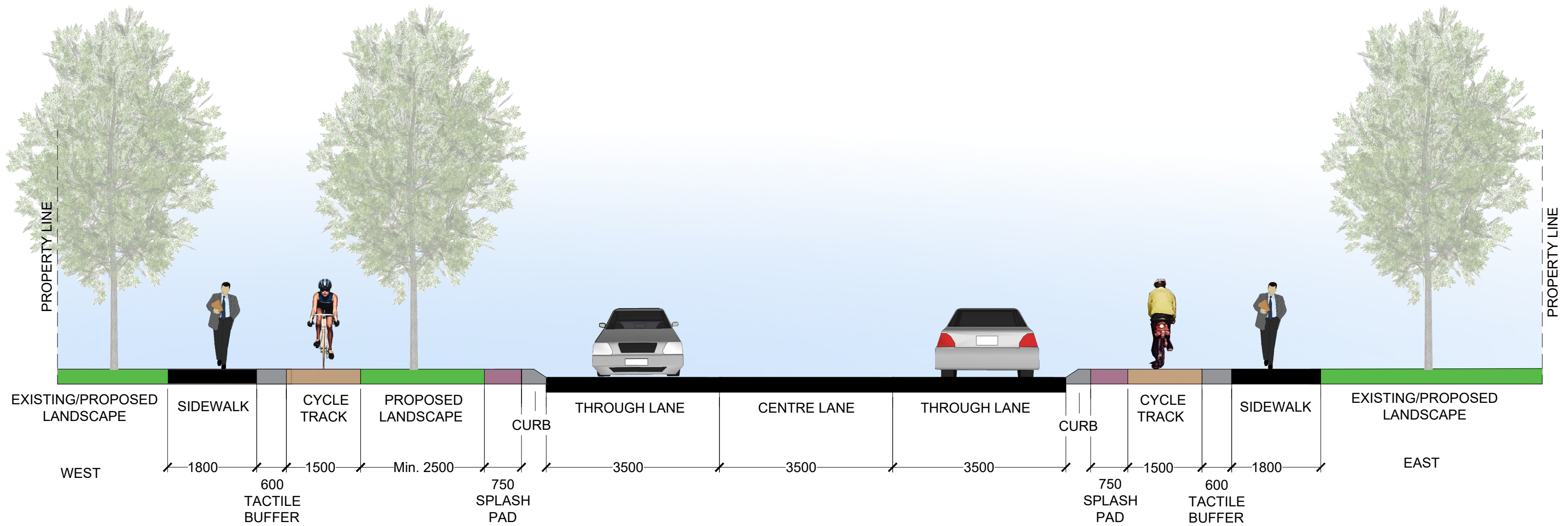
PREFERRED CROSS SECTION 1B-1B': BRITANNIA ROAD TO MATHESON BOULEVARD - LOOKING NORTH
