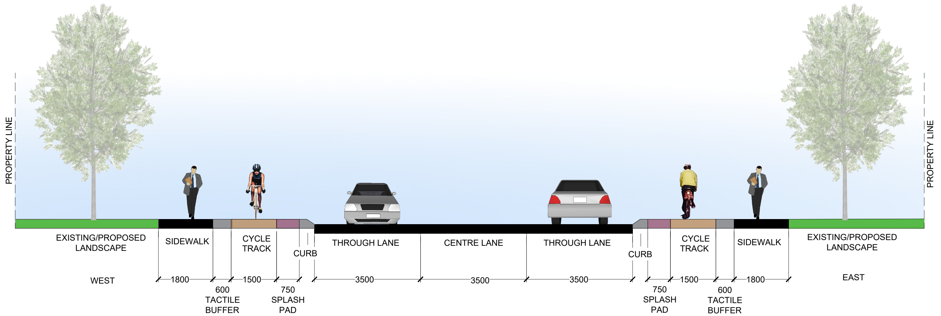
PREFERRED CROSS SECTION 1A-1A': BRITANNIA ROAD TO MATHESON BOULEVARD - LOOKING NORTH
