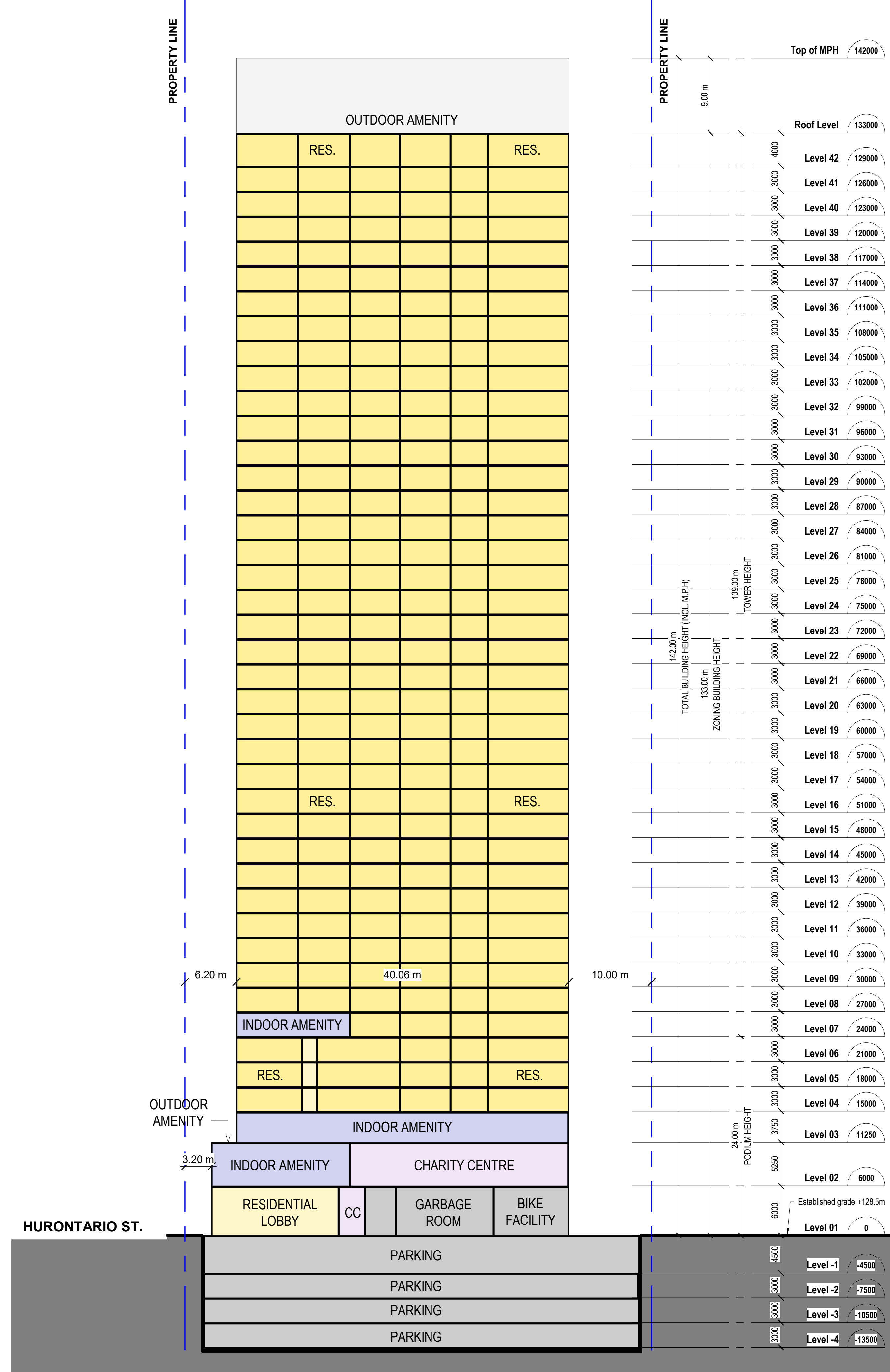
2 ZBA_Building Section_East AZ501 1 : 300
