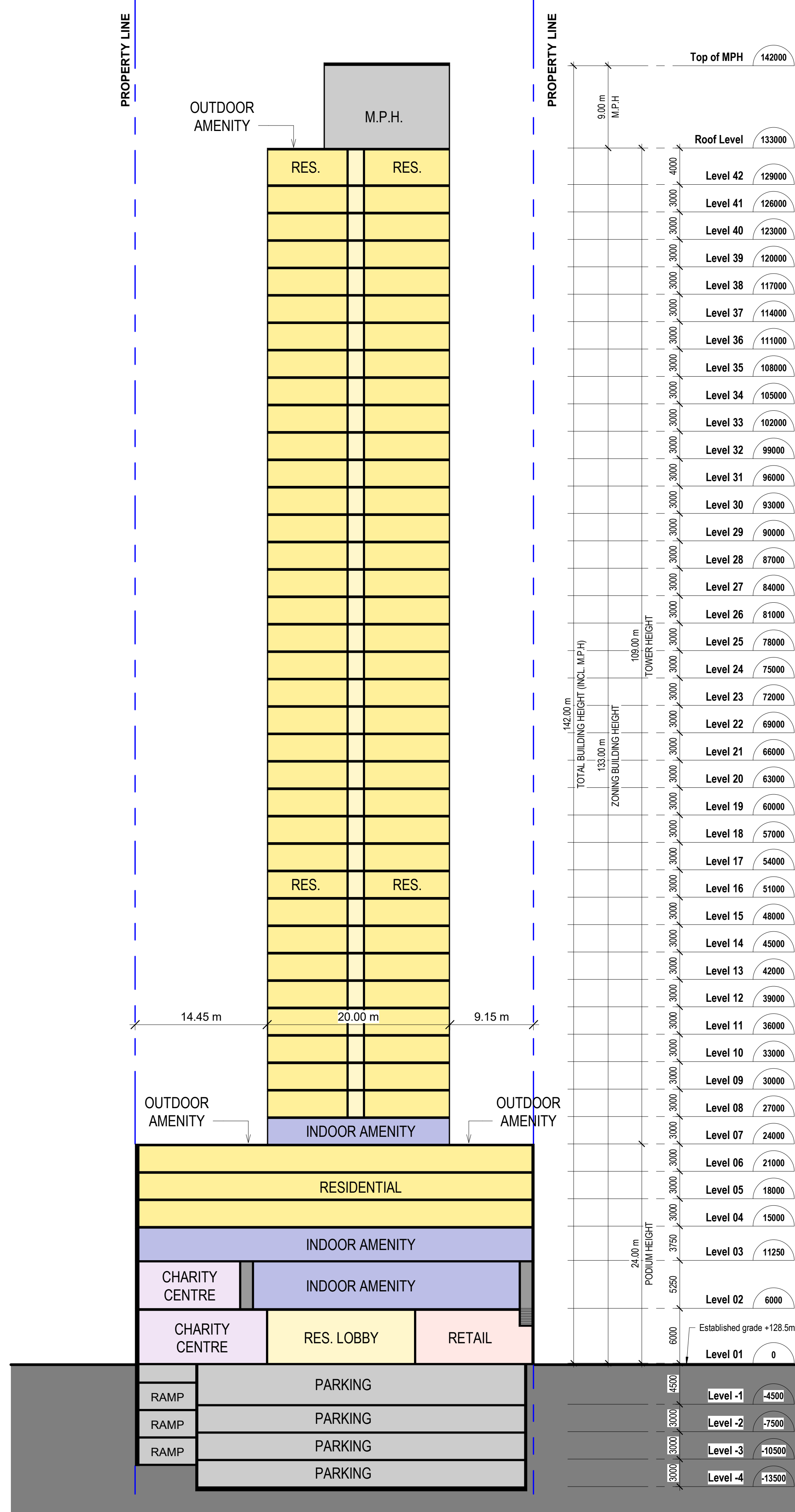
1 ZBA_Building Section_North AZ501 1 : 300
