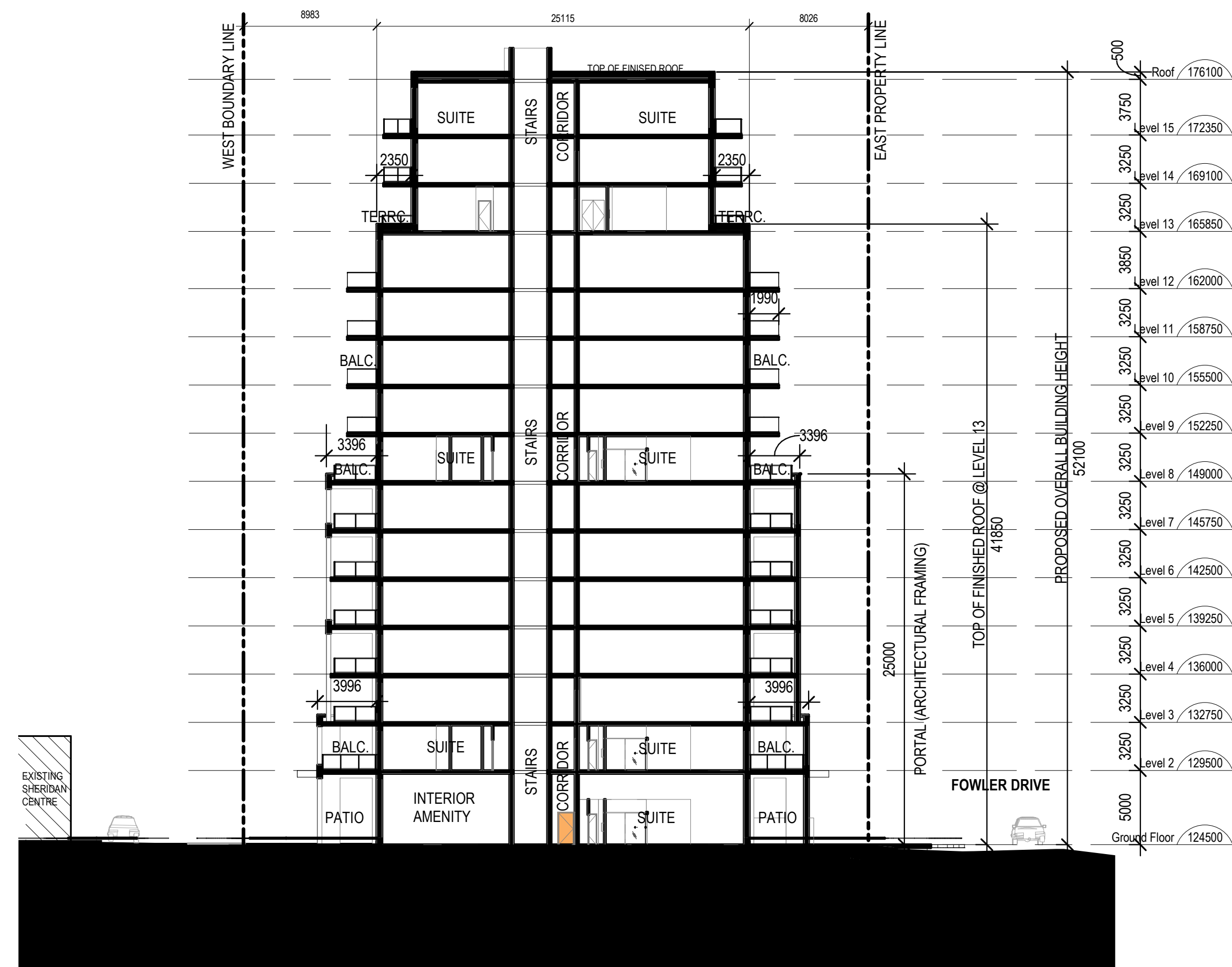
1 EAST WEST BUILDING SECTION A-200G 1:250
