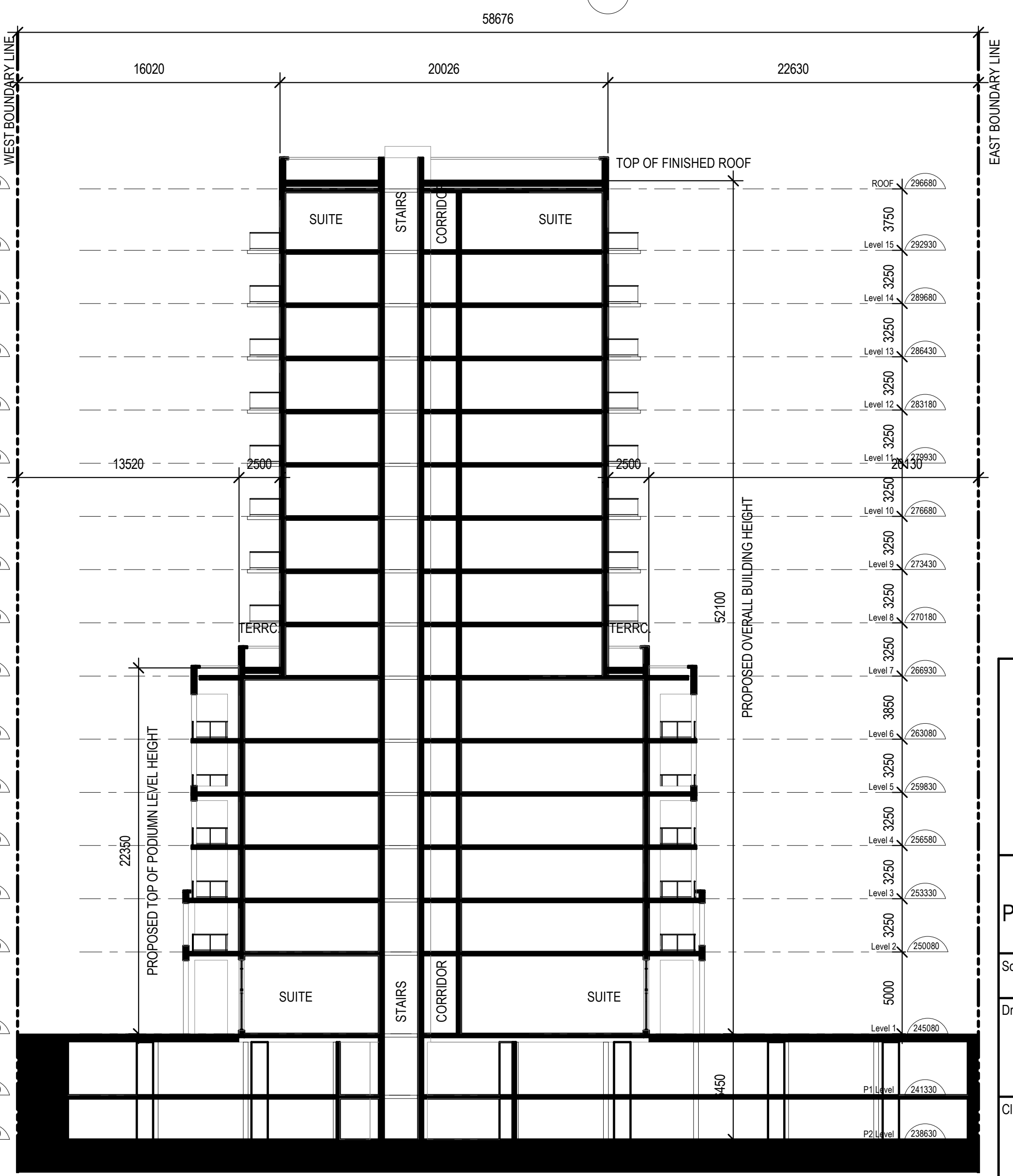
2 EAST WEST SECTION (RZ) A-201A 1:200
