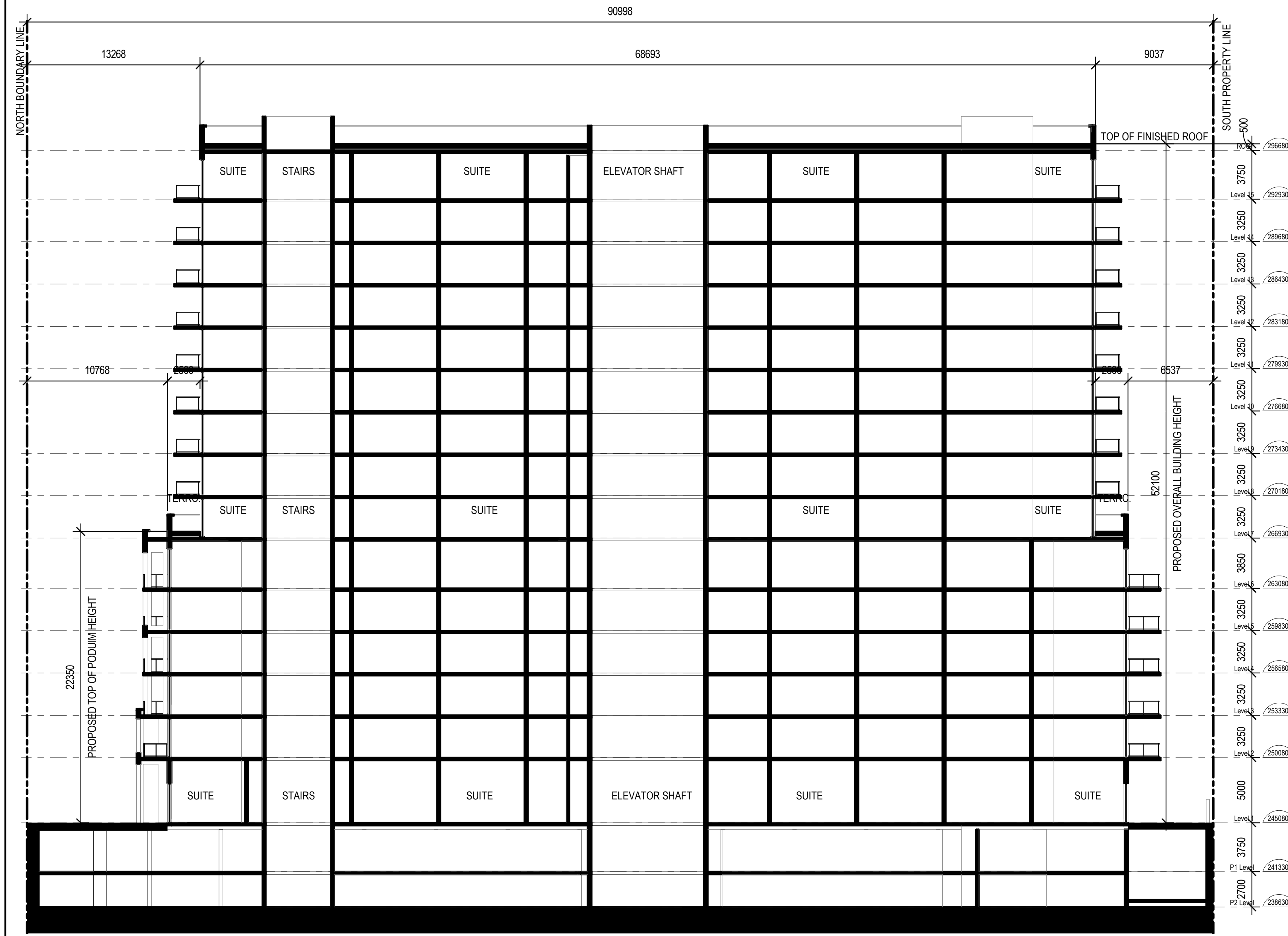
1 NORTH SOUTH SECTION (RZ) A-201A 1:200
