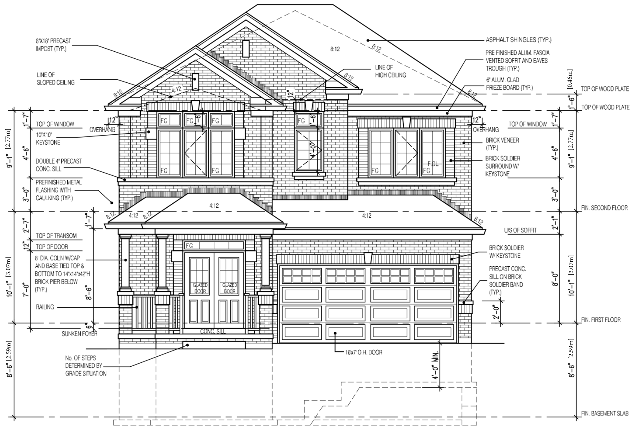
FRONT ELEVATION
