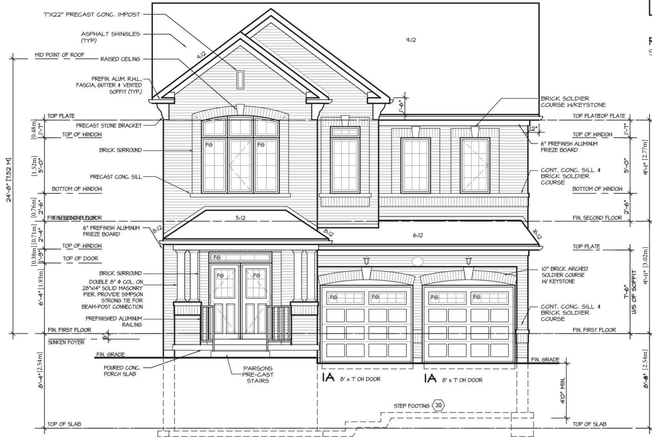
FRONT ELEVATION
