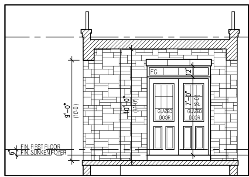
PORTICO INTERIOR ELEVATION
