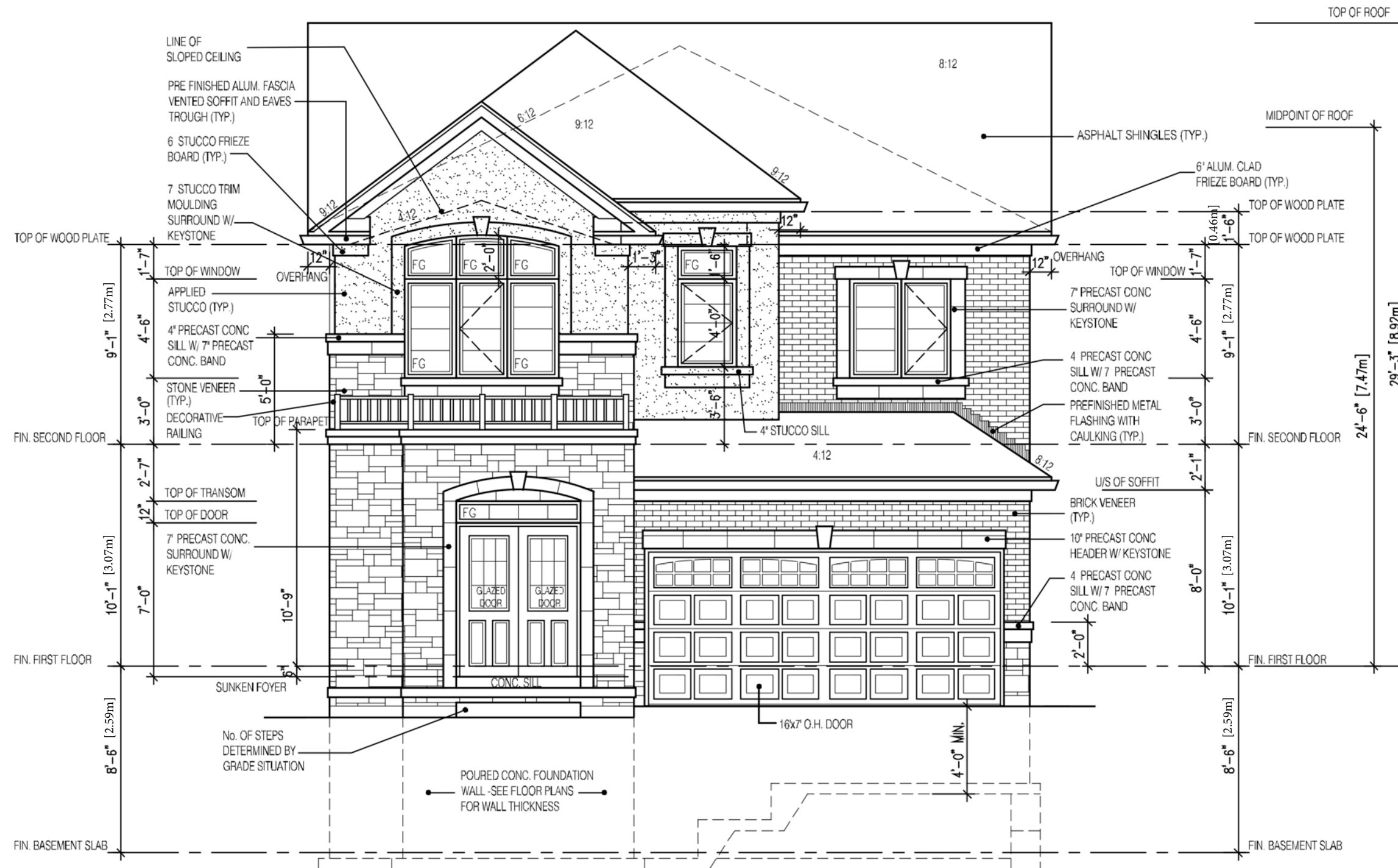
FRONT ELEVATION
