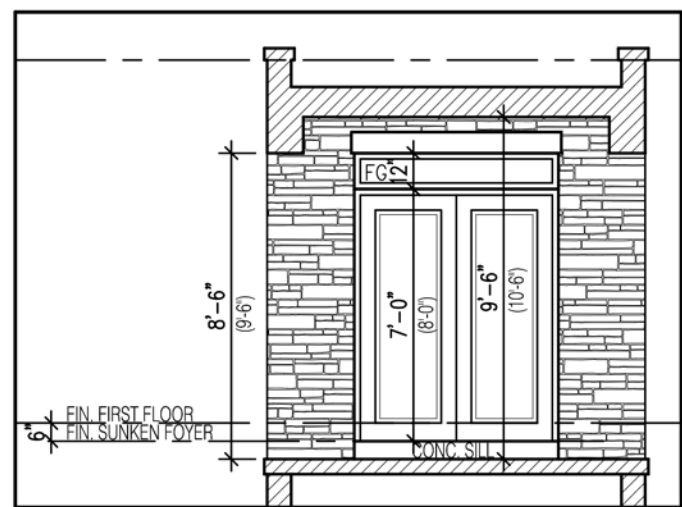
PORTICO INTERIOR ELEVATION
