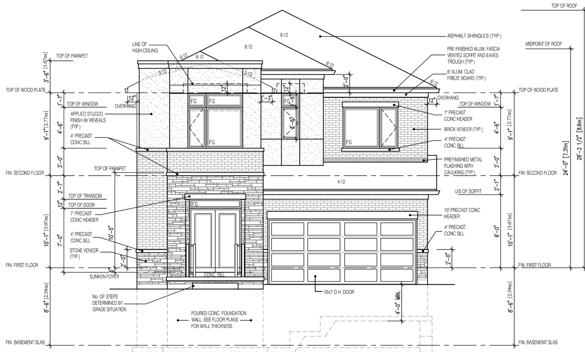
FRONT ELEVATION
