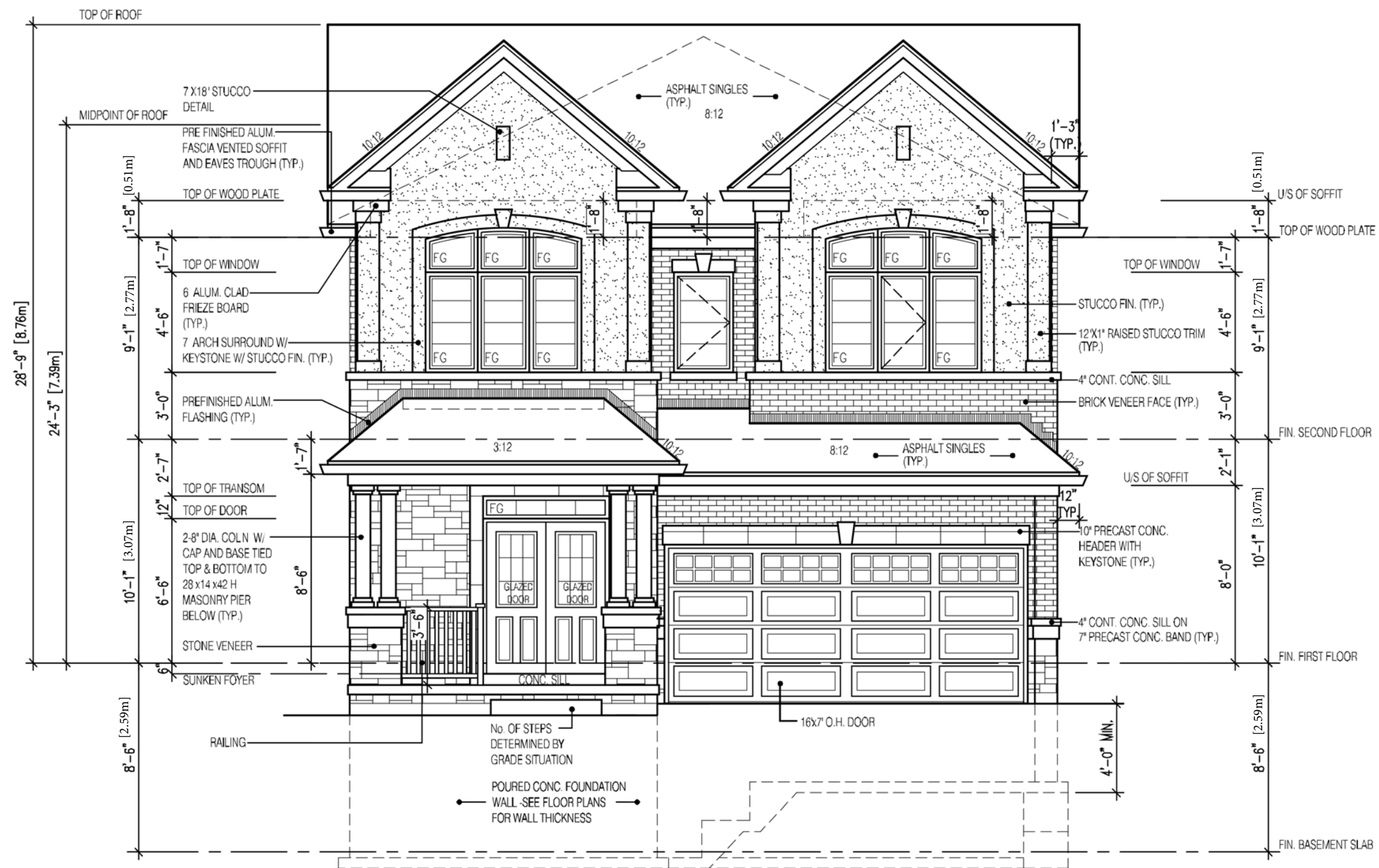
FRONT ELEVATION
