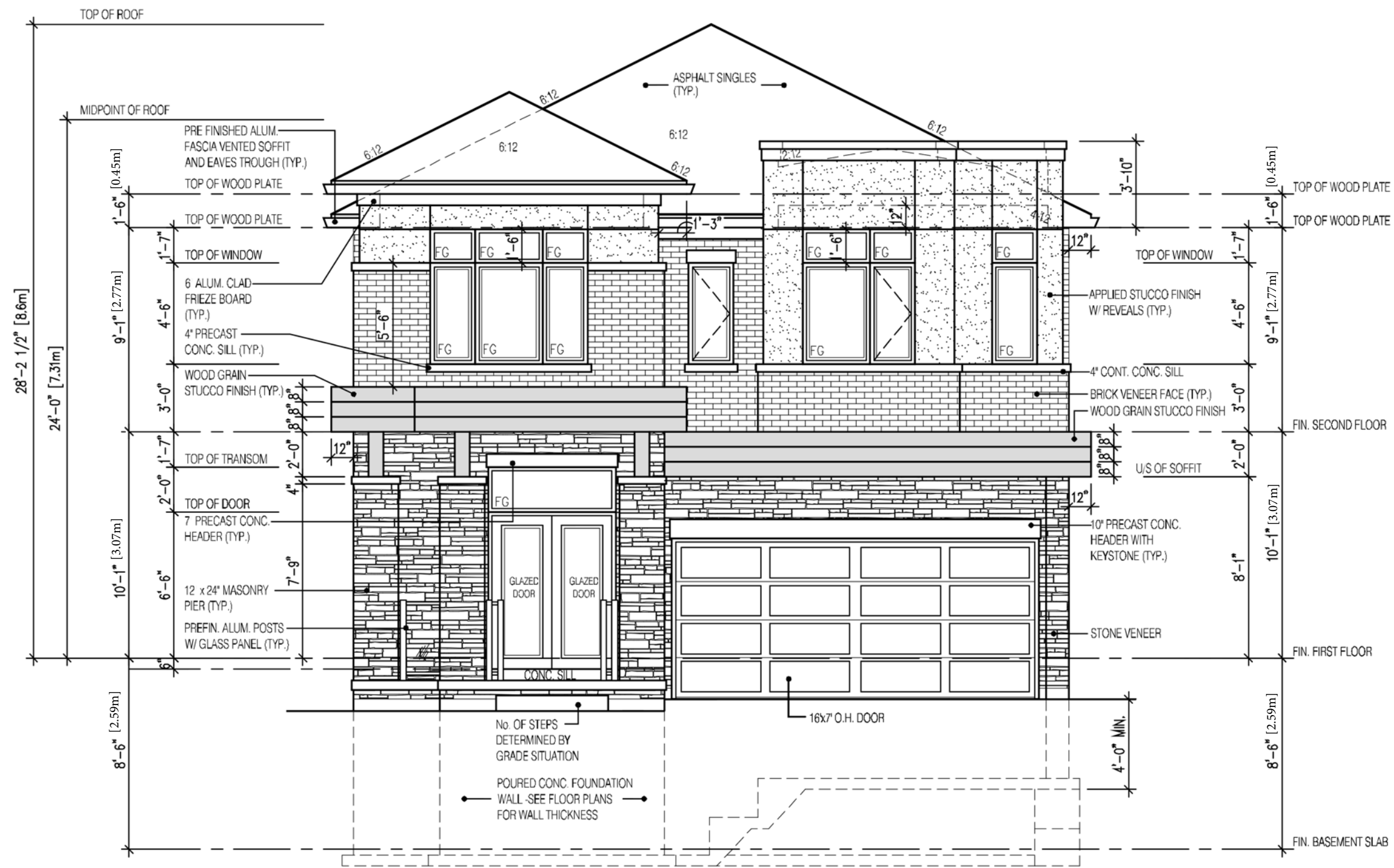
FRONT ELEVATION
