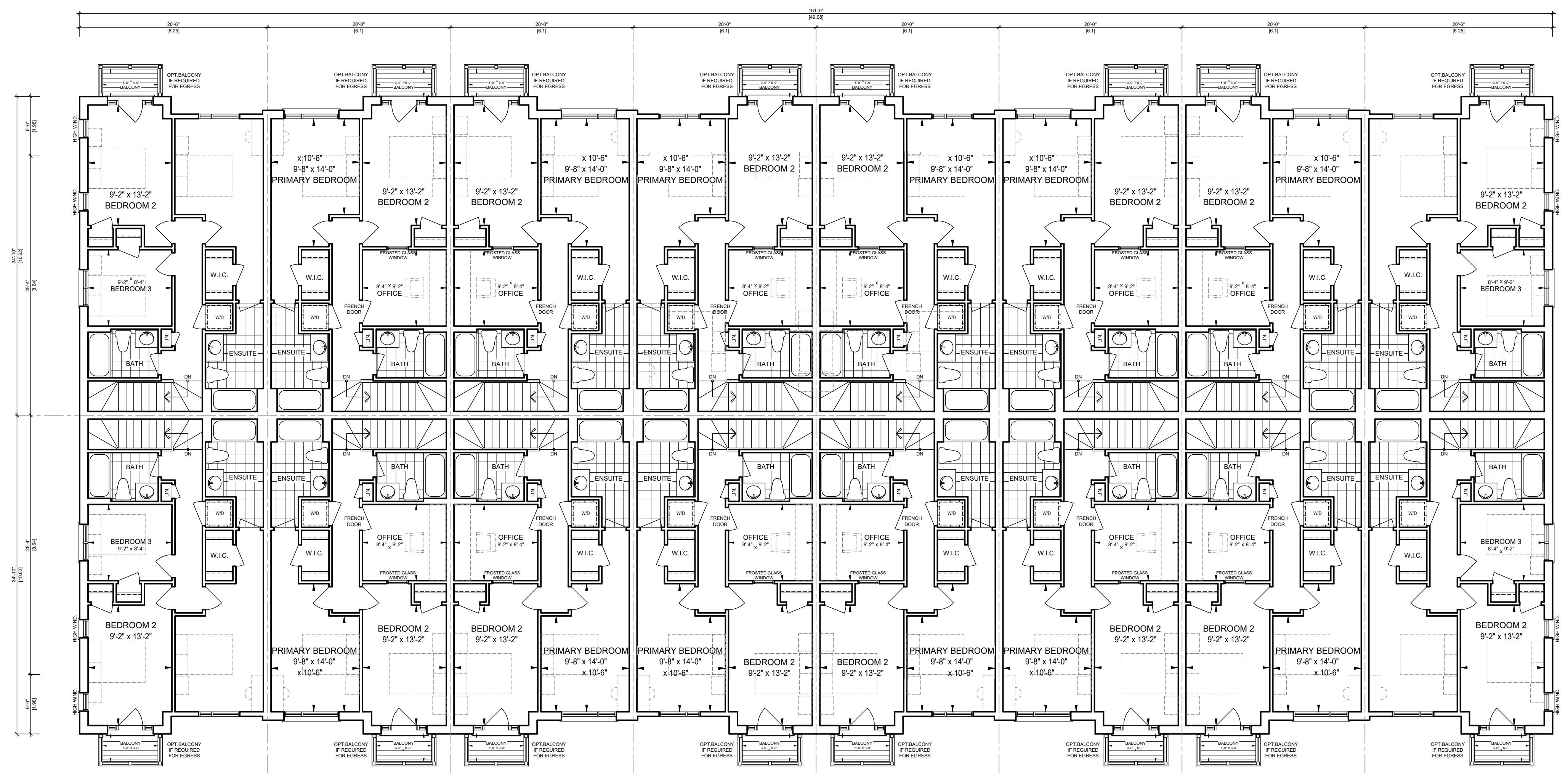
UPPER LEVEL FLOOR PLAN STYLE 'A'
