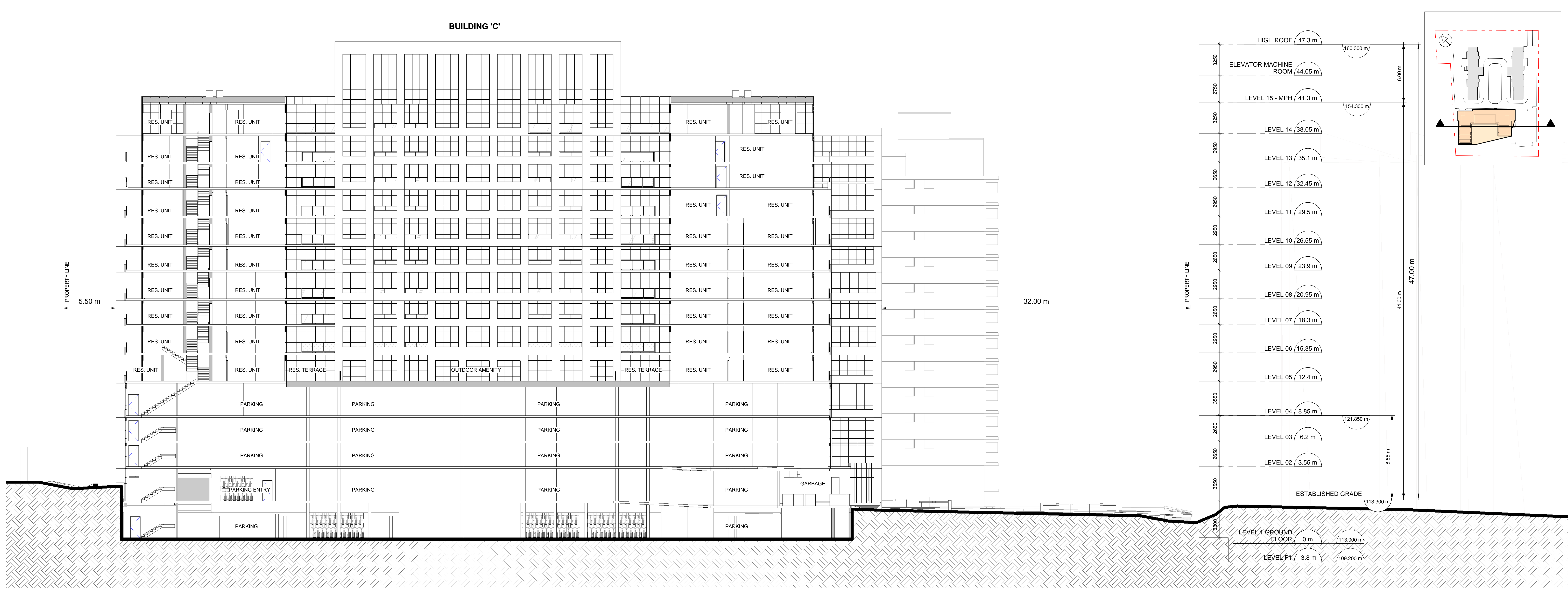
1 NORTH-SOUTH BUILDING SECTION Scale: 1: 150
