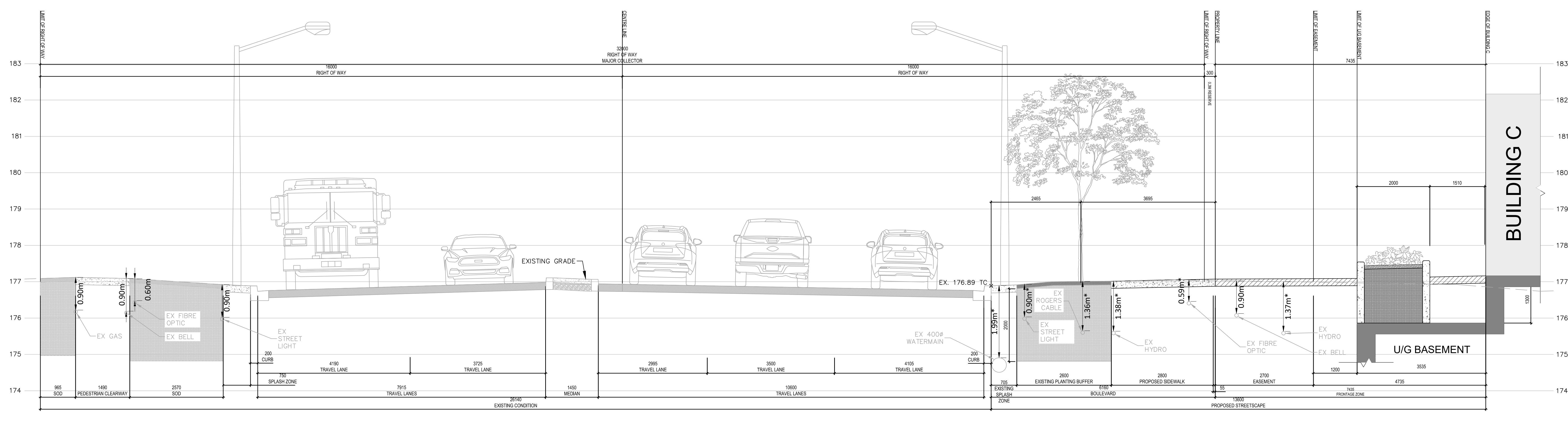
3 GLEN ERIN DRIVE - MAJOR COLLECTOR ROW SECTION AT BUILDING C - LOOKING NORTH CUP-1 SCALE: 1:50
