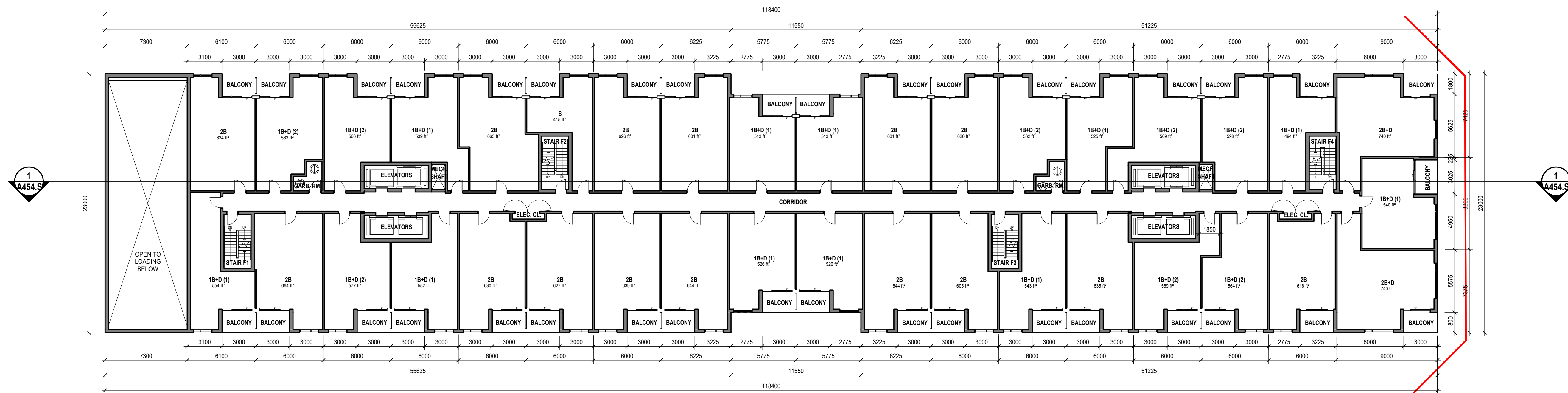
2 BUILDING F - FLOOR 2 A215.FS
