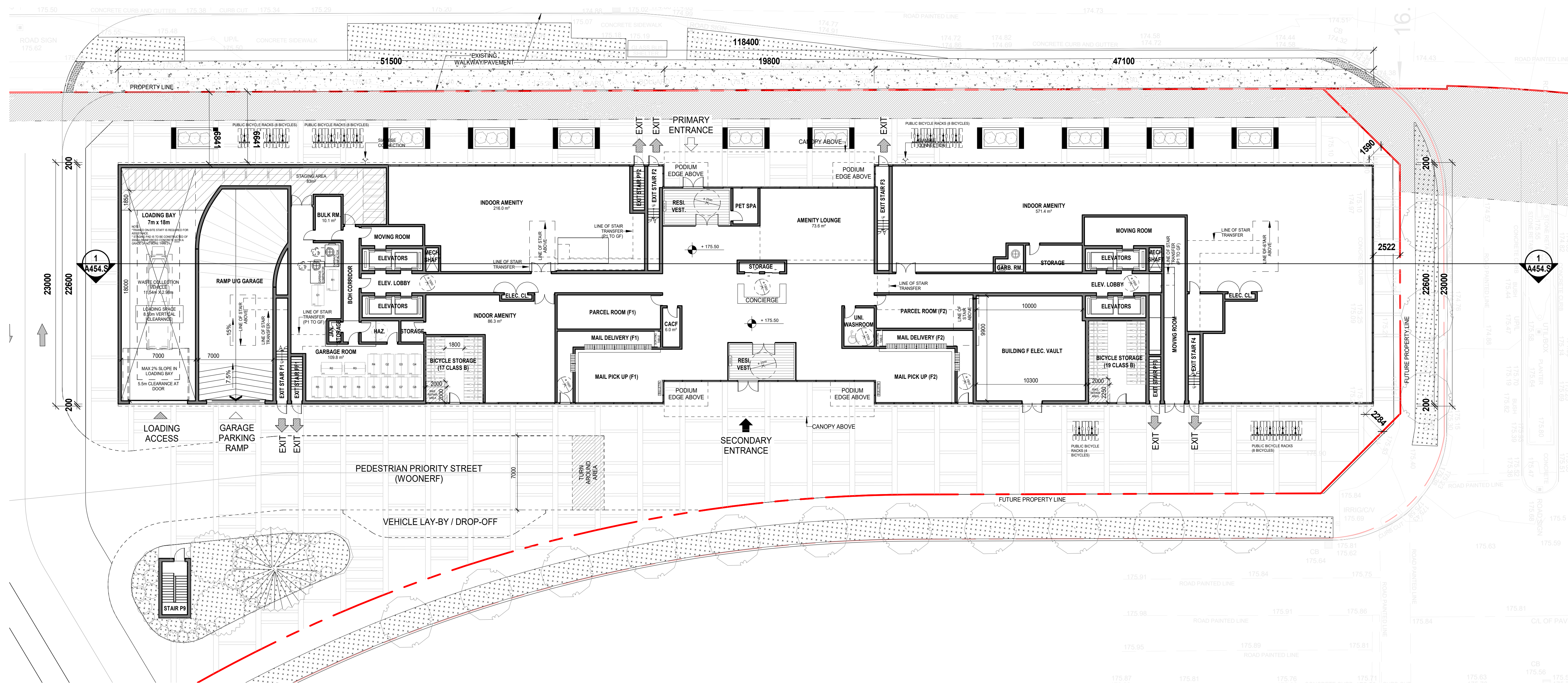
1 BUILDING F - GROUND FLOOR A215.FS
