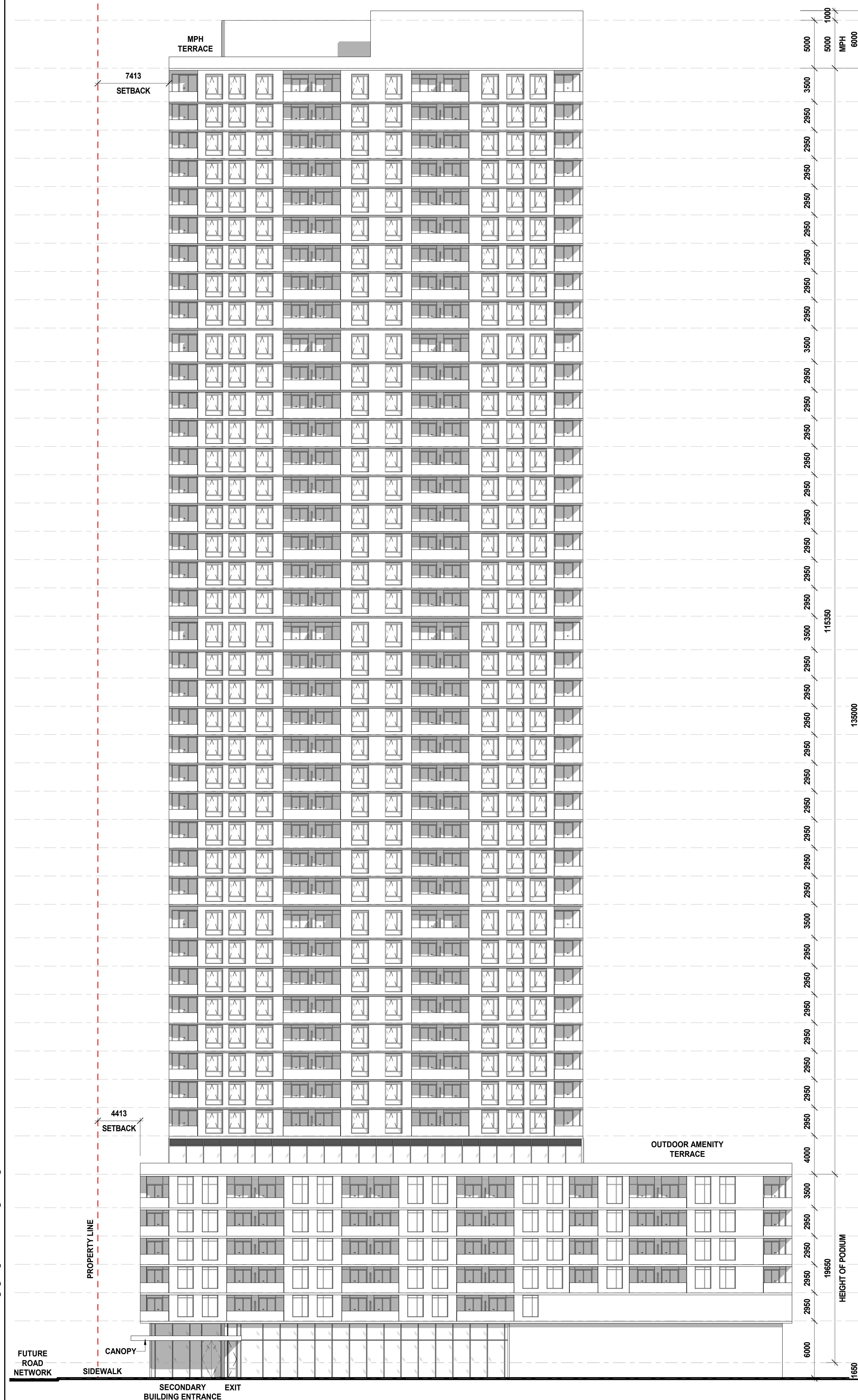
1 BUILDING G - PARKLAND SIDE ELEVATION
