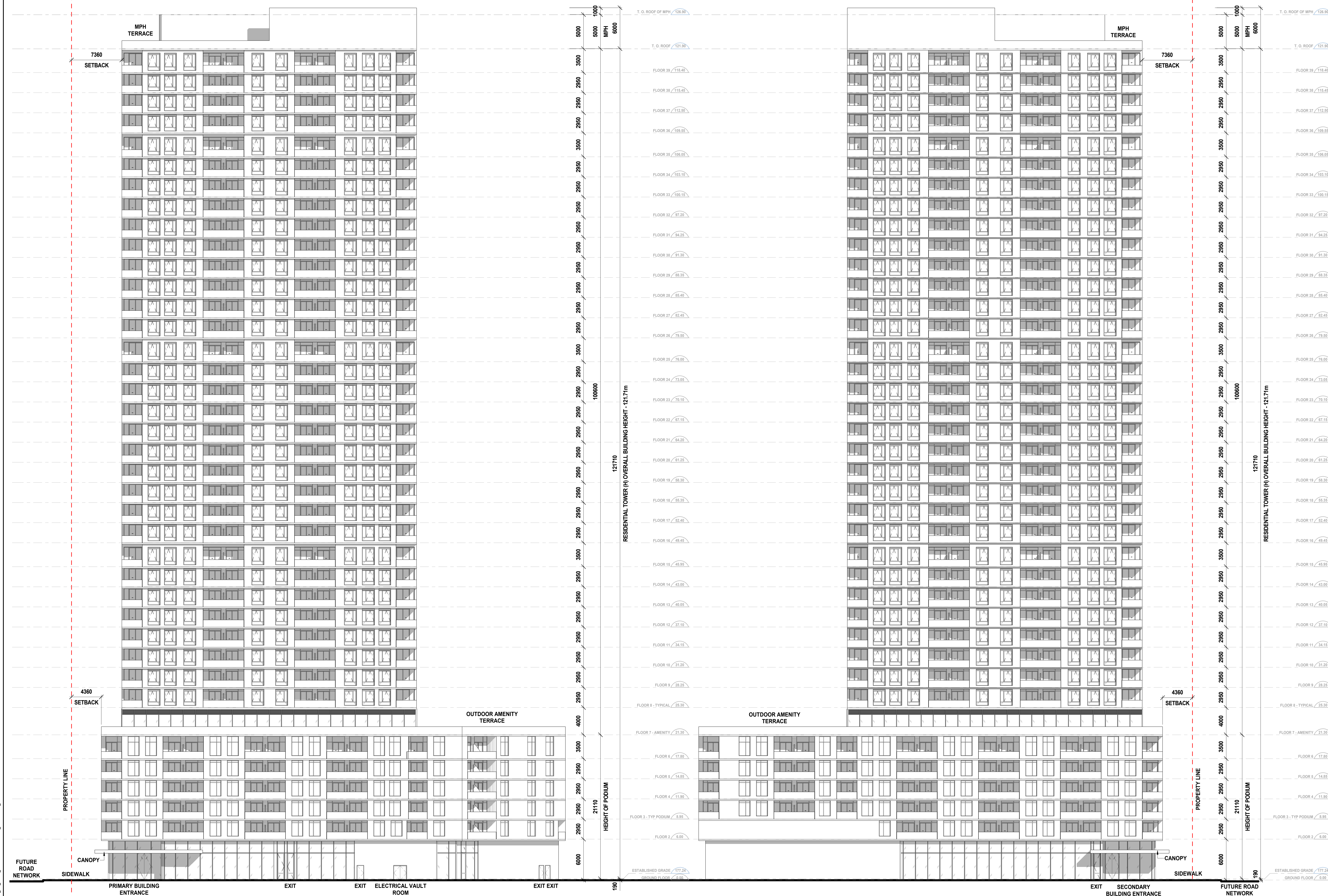
1 BUILDING H - PRIVATE DRIVEWAY SIDE ELEVATION
