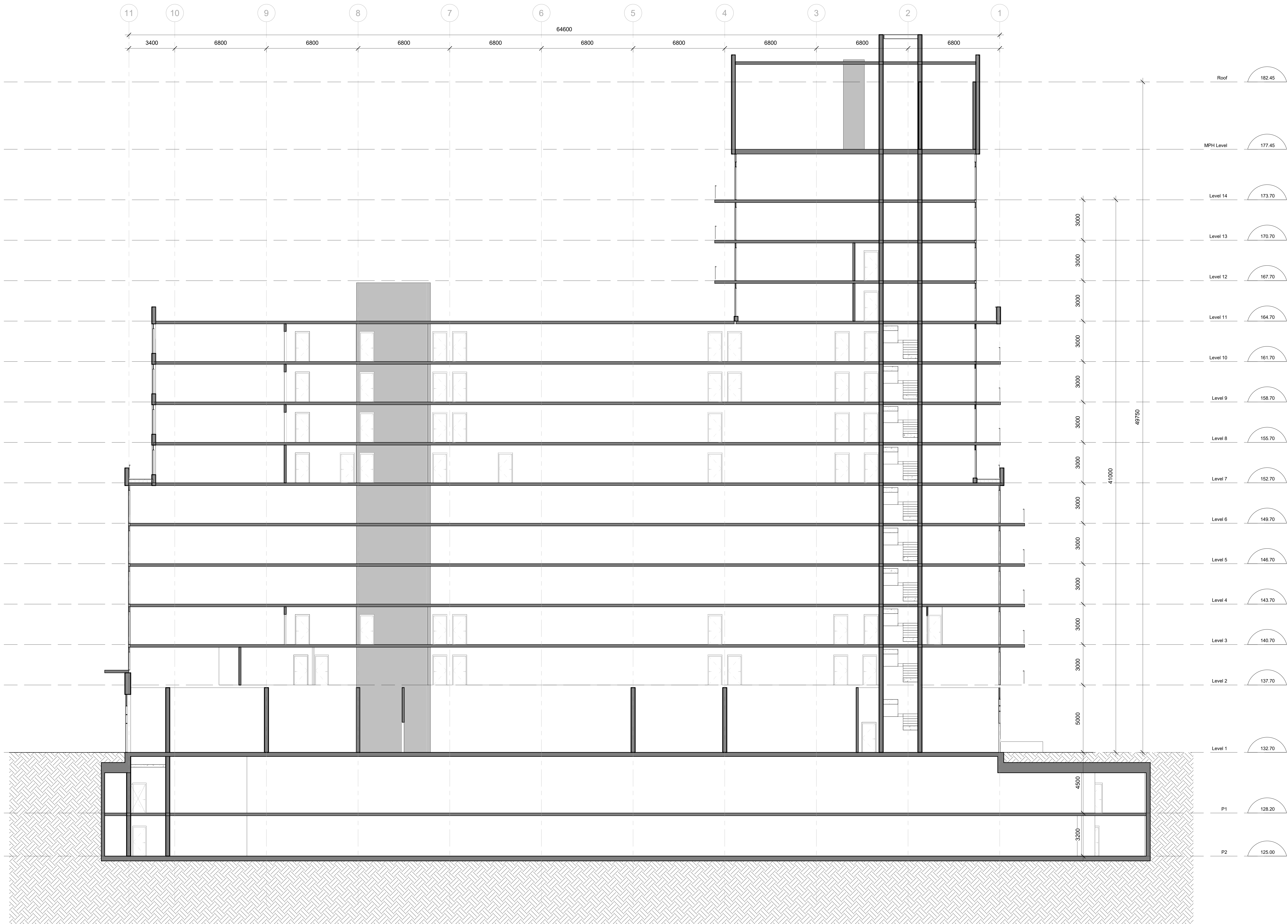
1 Longitudinal Building Section 1 : 100
