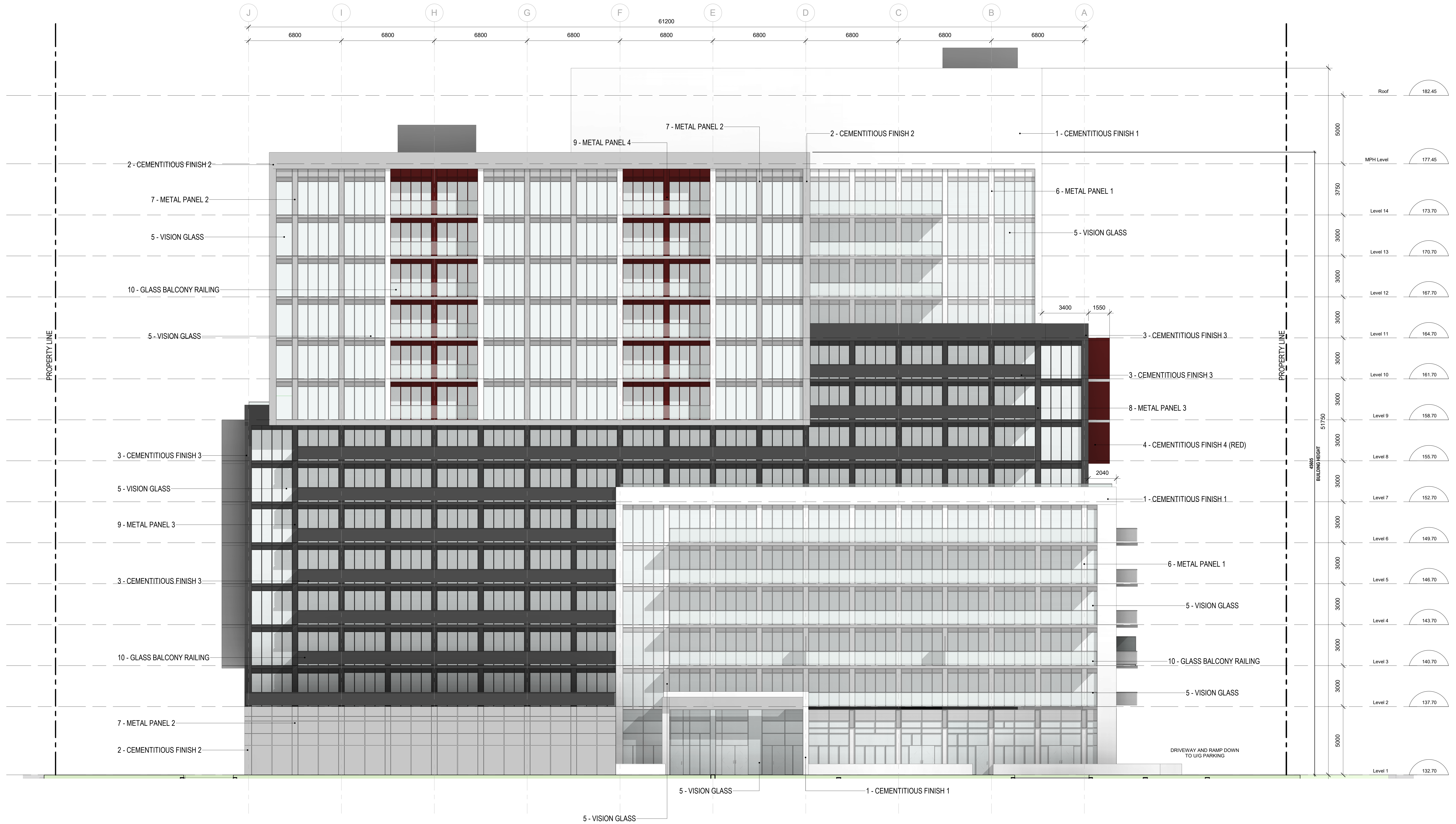
1 North Elevation 1 : 100
