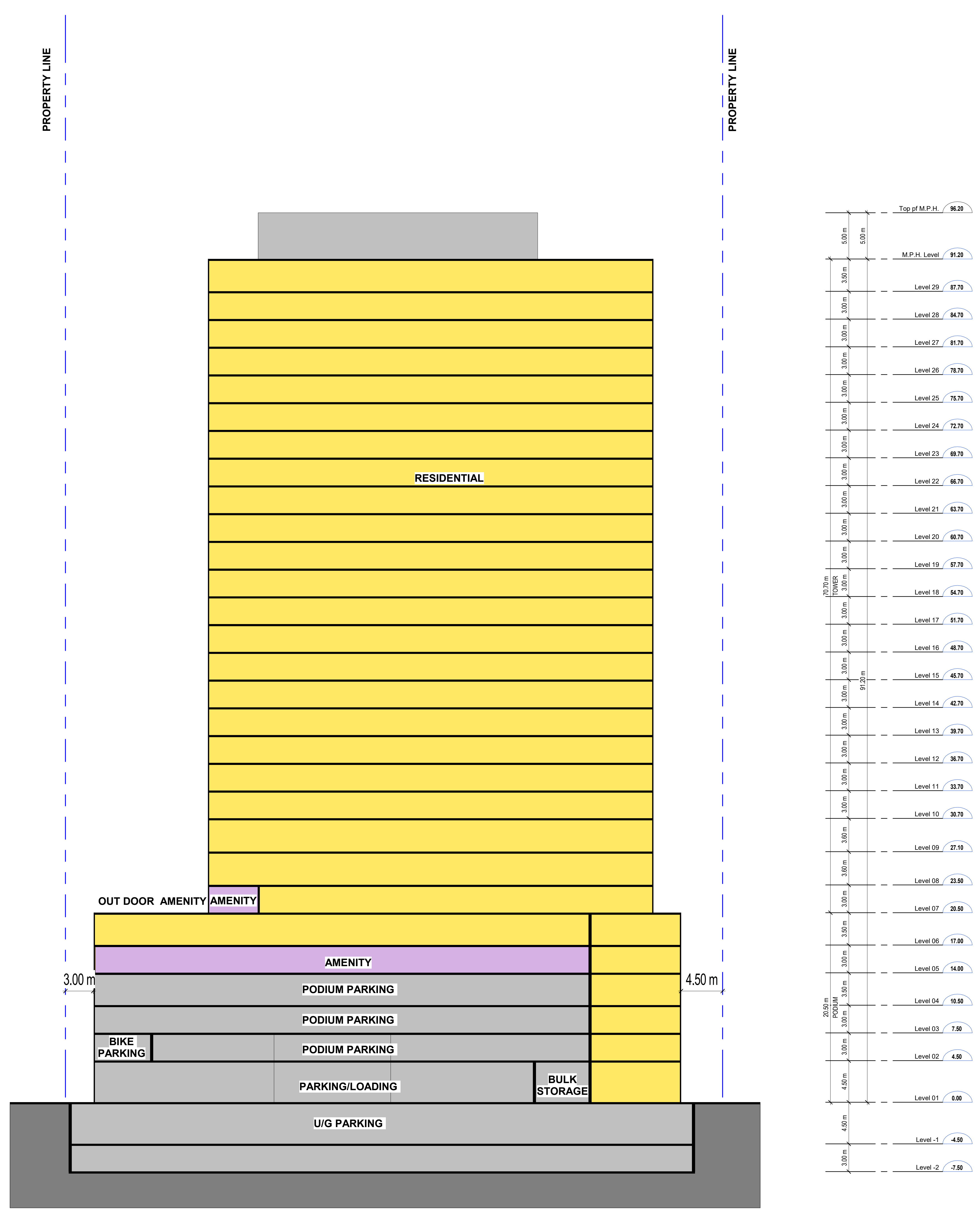
2 ZBL_E-W Section AZ501 1:200
