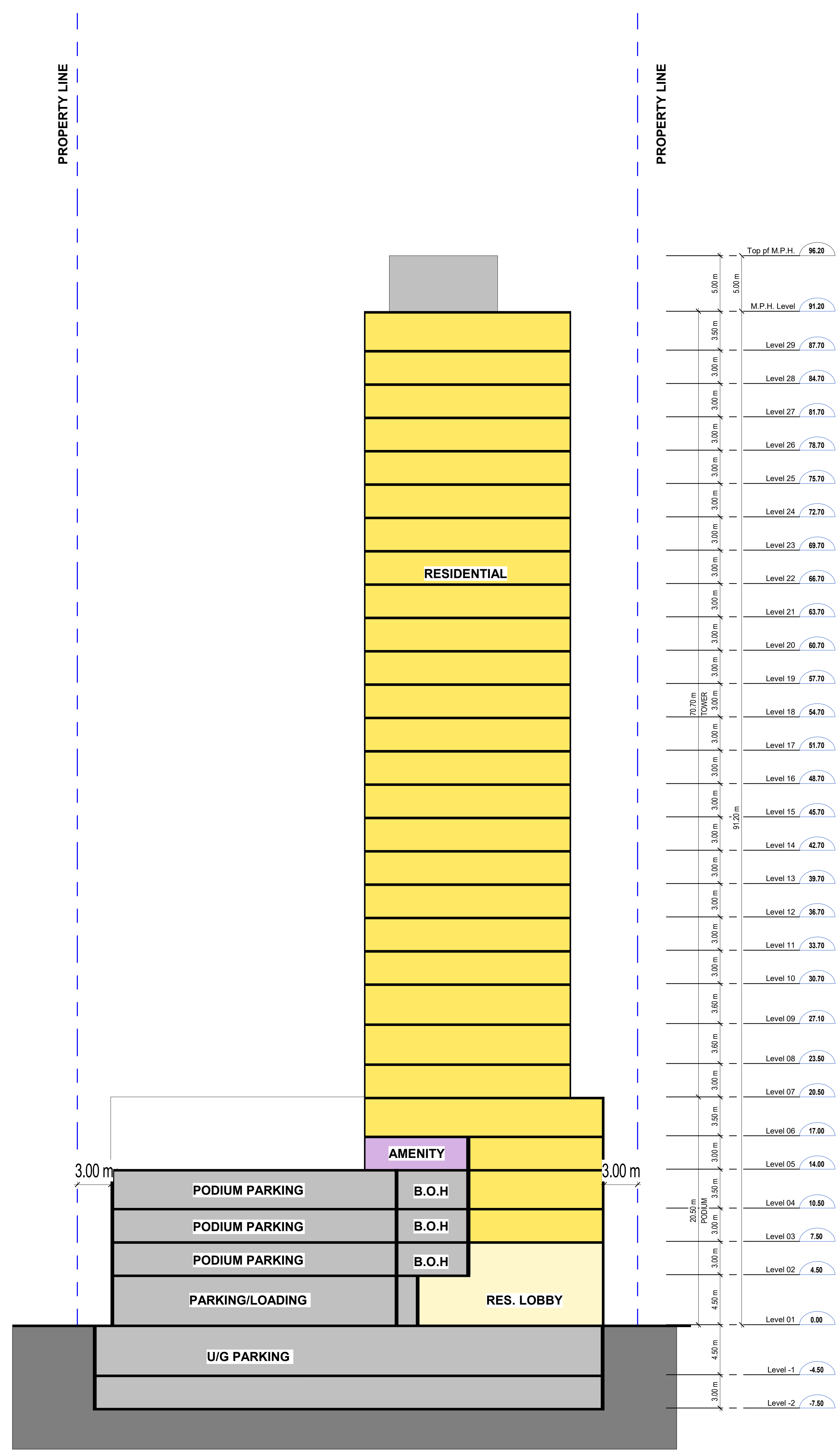
1 ZBL_N-S Section AZ501 1:200
