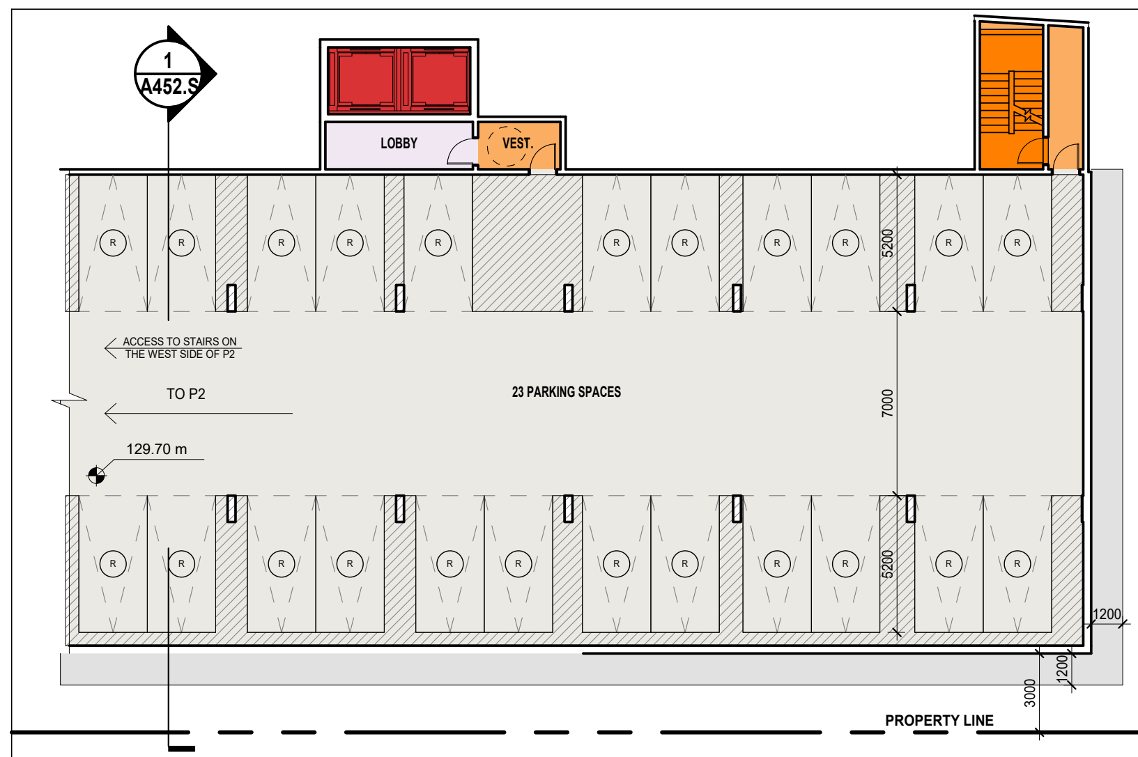
2 A102.S P2 Lower Underground Plan
